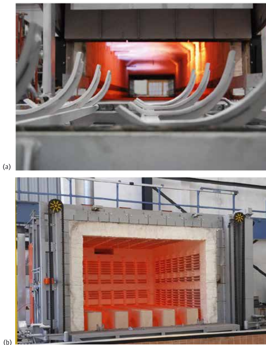
Figure 1. (a) Fossil Fueled Industrial Furnaces, (b) Electrical Industrial Furnaces
